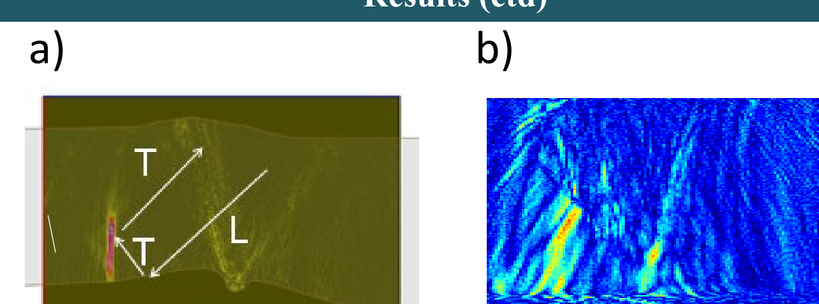
Figure 3. The back wall crack imaged (using the half-skip LTT mode) with a) CIVA and b) the AutoNDE code.
